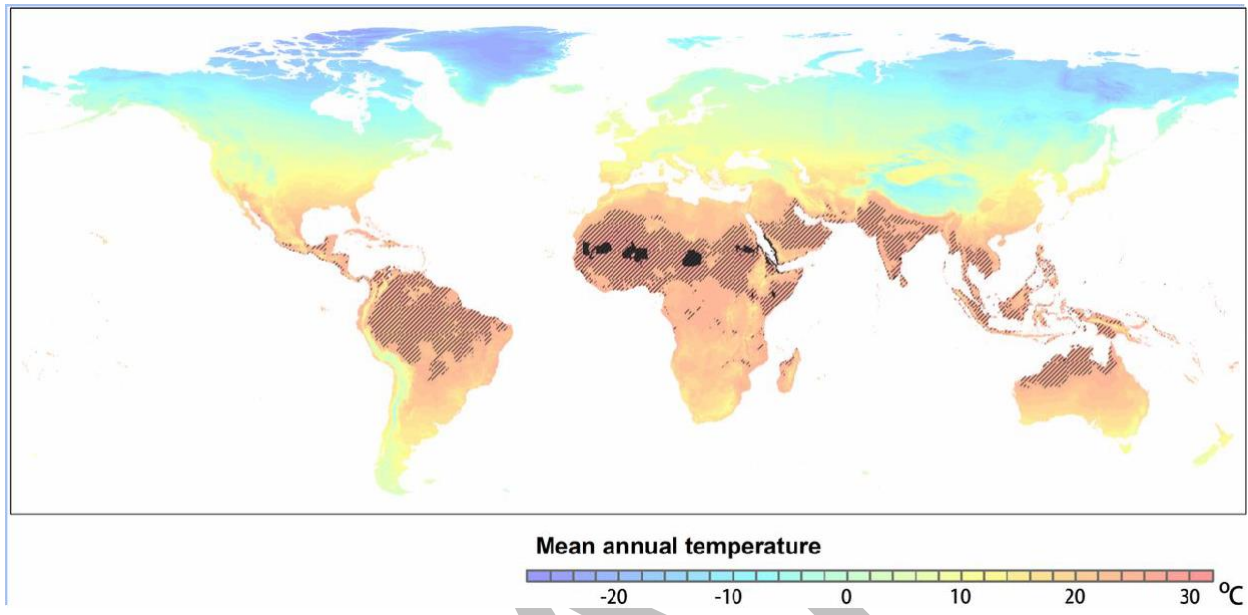
Figure IV-1. Expansion of extremely hot regions in a business-as-usual climate scenario. Today, mean annual temperatures (MATs) >29^{\circ}\text{C} ( 84.2^{\circ}\text{F} ) are restricted to the small dark areas in the Sahara region (0.8% of global land area). With continued emissions these conditions are projected to occur throughout the shaded area (19% of global land area) by 2070, currently home to 3.5 billion people. Background colors represent current MATs. 139
